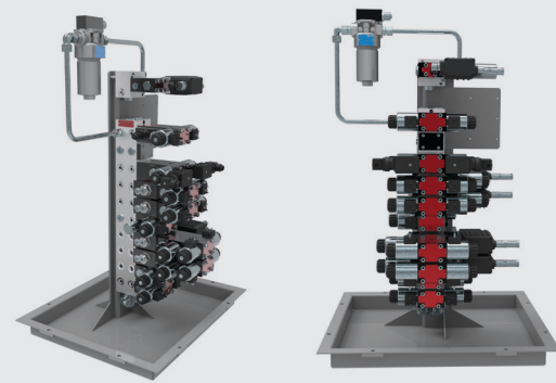
1 Custom manifolds
