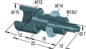
BV12SC Side Load Adaptor
