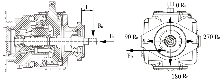
Diagram of external radial shaft loads
