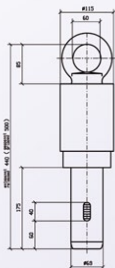
Dimension drawing AL 70/76
