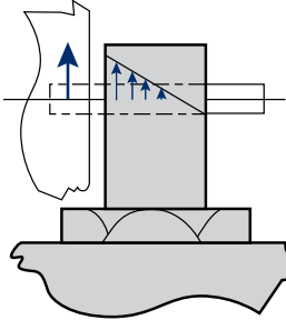
Figure 2 Cantilevered mount
